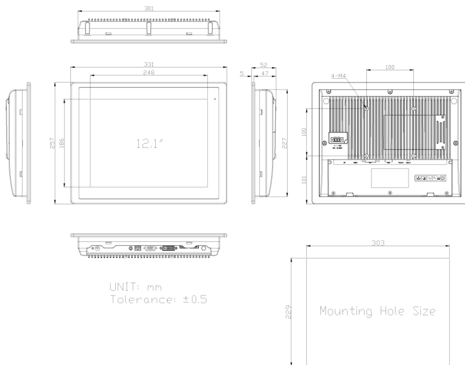
Figure 1.3: Dimensions of FABS-112PRG(H)
