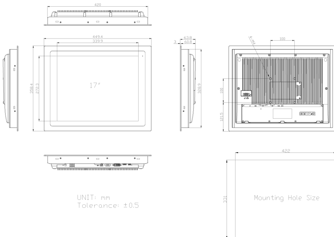
Figure 1.6: Dimensions of FABS-117PRG(H)
