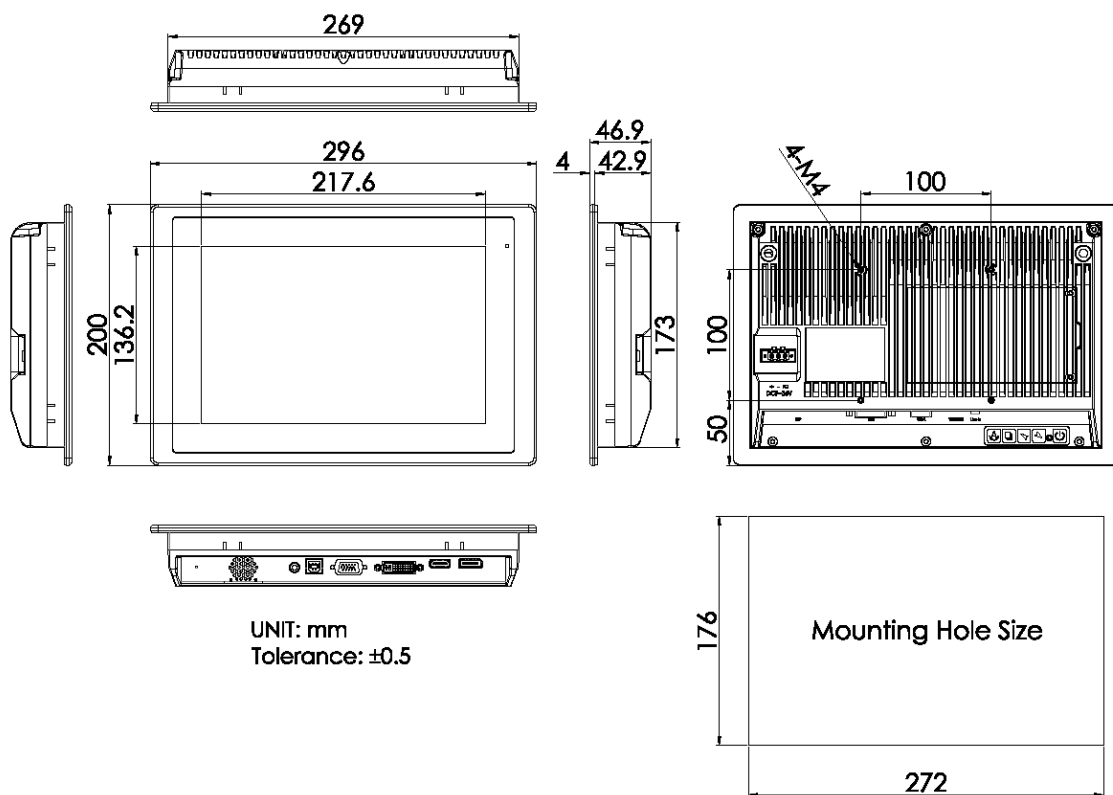
Figure 1.2: Dimensions of FABS-110PRG(H)
