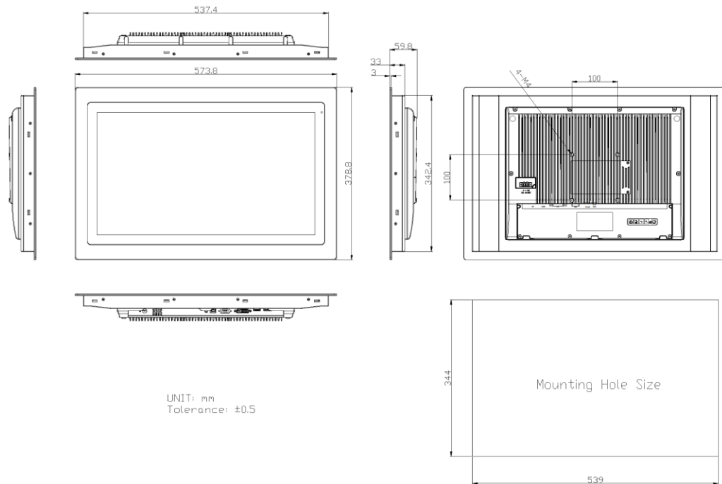
Figure 1.9: Dimensions of FABS-121PRG(H)
